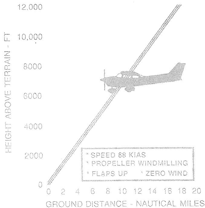
Figure 4 Maximum Glide
